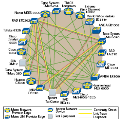
Figure 10: End-to-End Service OAM Tests (CFM)
